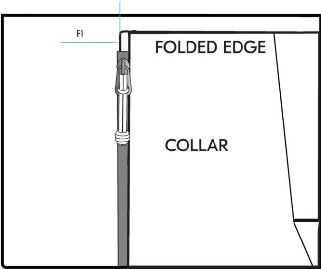
Option B, zipper stop 0,5 cm below CHINGUARD windfalp top end.
